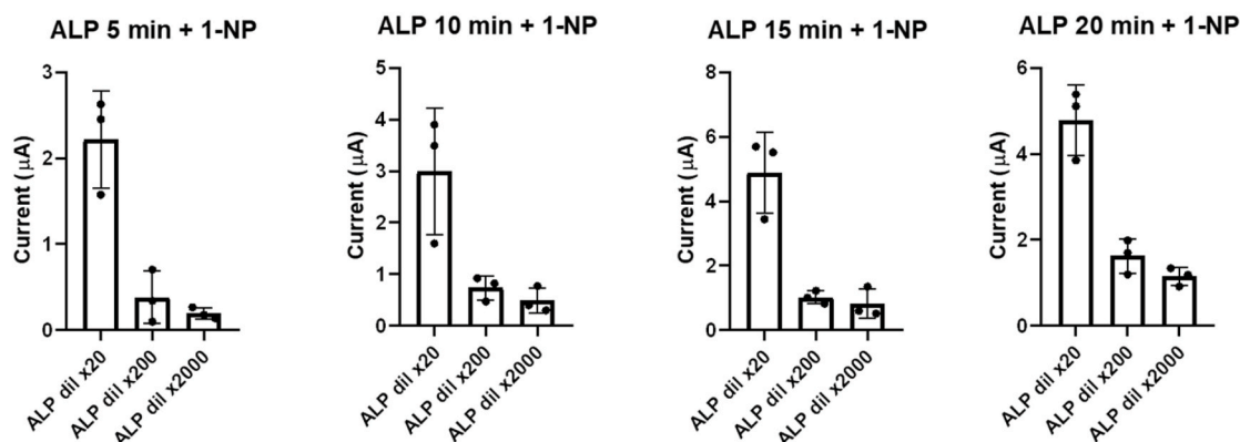
Fig. 4. Characterization of rGO electrodes on nitrocellulose with ALP-based enzymatic approach. Dilutions of the ALP stock solution (x20, \times 200 and \times 2000 ) were studied to assess the potential of ALP to provide an analytical signal in electrochemical LFA. (A) Differential pulse voltammograms after mixing ALP with a fix concentration of 1-NP (5 mM). Column graphs represent the peak height at every 5 min after mixing. Experiments were performed in triplicate. (B) Peak height of the same differential pulse voltammograms as a function of ALP dilution factor.
